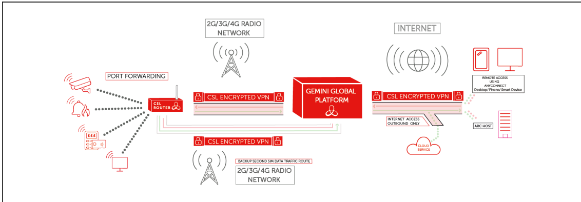
Figure 2 - 4G Primary Network Diagram
